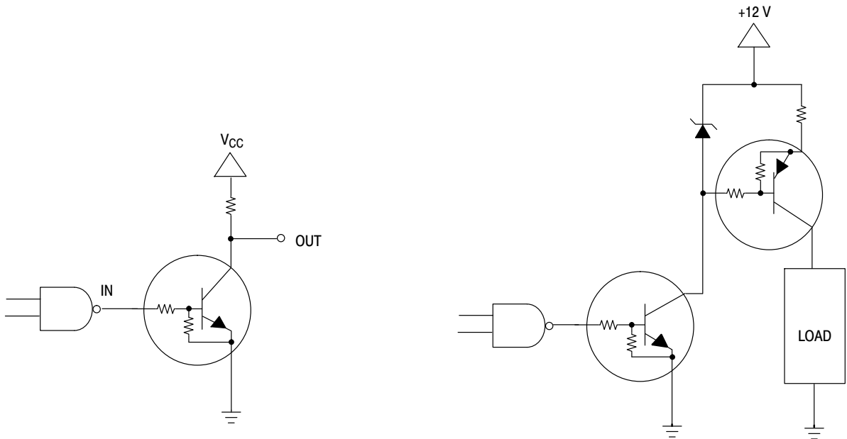
Figure 28. Open Collector Inverter: Inverts the Input Signal
